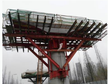
Overpass box girder formwork
