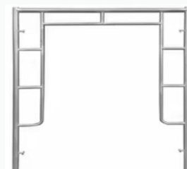
Walk-through frame Φ42.5*2.4mm
