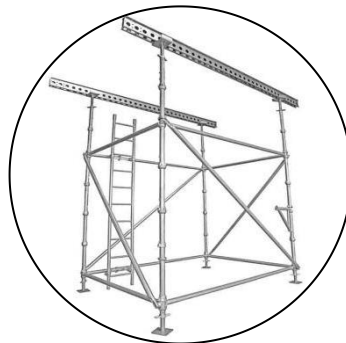
Side bracket Φ48.3*3.2mm
