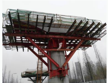
Overpass box girder formwork
